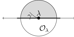
Figure 4.1. Outgoing spectral singularity located inside the essential spectrum. The figure shows an example of a curve \gamma : (0, 1] \rightarrow \mathcal{O}_\lambda^+ , where \mathcal{O}_\lambda^+ = \mathcal{O}_\lambda \cap \mathbb{C}^+ and \mathcal{O}_\lambda is a complex neighborhood of \lambda . The thick line represents the essential spectrum of H .
