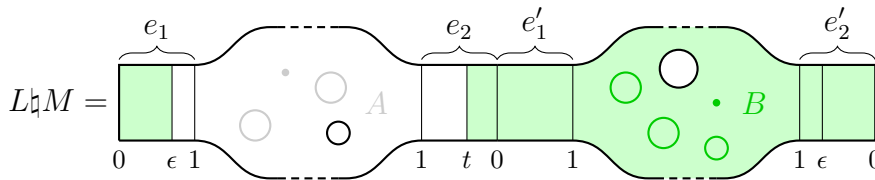
Figure 1.4. The submanifold M_{\epsilon,t} (shaded in green) of L\mathfrak{h}M from the proof of Theorem 1.55.
