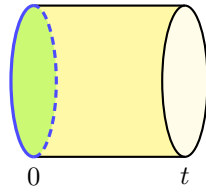
Figure 1.1. An illustration of the notation for the solid cylinder \mathbb{B}_t^d from Notation 1.9 for d = 3 . Its lower boundary \partial_l \mathbb{B}_t^3 is coloured yellow, its base b\mathbb{B}_t^3 is yellow-green and the codimension-2 stratum \partial(b\mathbb{B}_t^3) = \partial\mathbb{D}^2 \times \{0\} is blue.
