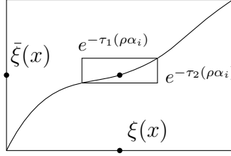
Figure 1.3. The image of the cone type \alpha_i \mathcal{C}_\infty^c(\alpha_i) by the graph curve \mathcal{G} in the C^{1+\nu} -torus \partial\Omega \times \partial\Omega^* .
