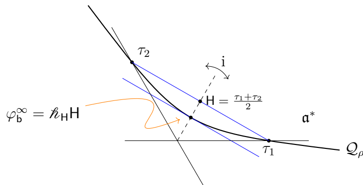
Figure 1.4. The critical hypersurface of a strictly convex projective structure on S . Since \mathbf{H} is a convex combination of \{\tau_1, \tau_2\} one has \|\mathbf{H}\|^1 = 1 and thus \|\varphi_{\mathfrak{b}}^\infty\|^1 = \mathfrak{h}^{\mathbf{H}} .
