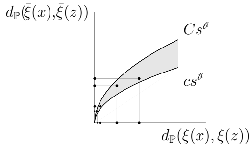
Figure 1.1. A \varrho -concave point x . The marked points on the axis' represent d_{\mathbb{P}}(\xi(x), \xi(y_k)) and d_{\mathbb{P}}(\bar{\xi}(x), \bar{\xi}(y_k)) respectively.
