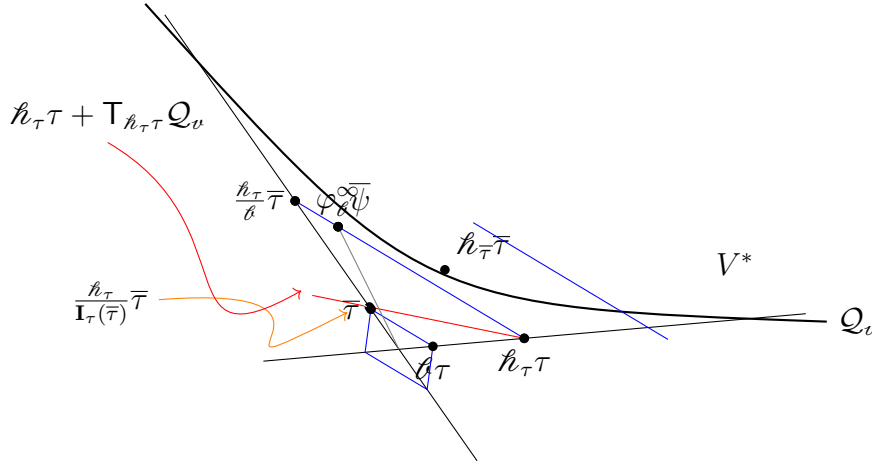
Figure 5.1. The situation of Lemma 5.9.
