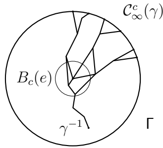
Figure 4.1. The coarse cone type at infinity, picture from [PSW23].
