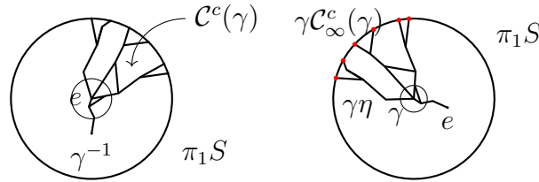
Figure 1.2. The coarse cone type of \gamma \in \Gamma (left). The set \gamma \cdot \mathcal{C}_\infty^c(\gamma) (right). Pictures from [PSW21].
